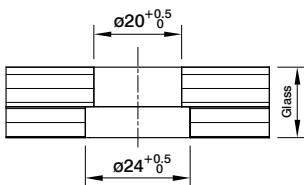
Glass Drilling
